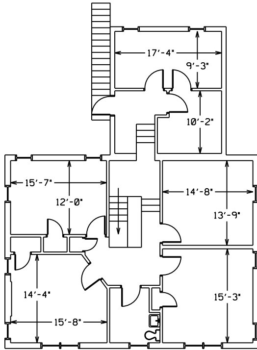
SECOND FLOOR 1,686 SF
